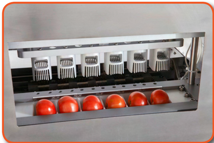
MCT 5 Tomato Slicer slices 6 tomatoes per cycle.
